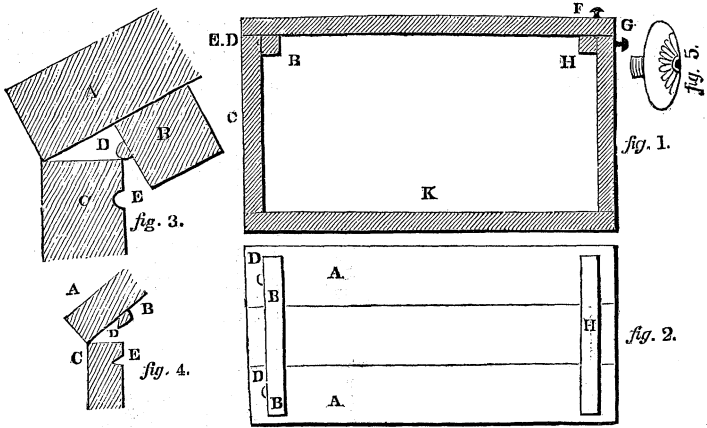
285. Fig. 1. Section of the box. A, the lid. K, the bottom. C, D, the two sides. 2. The inside of the lid. B, H, cross-bars nailed inside the lid. Found at Thebes.
